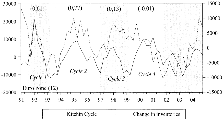
Fig. 1 European short-term growth cycle
