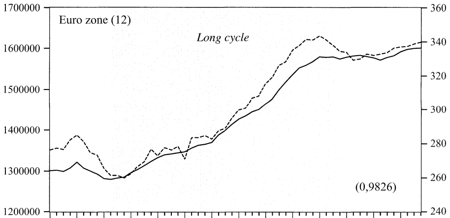
Fig. 2 European long-term growth cycle
